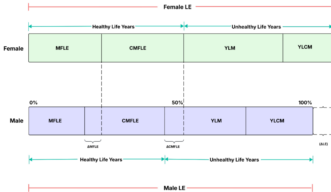
Figure 1: Framework
